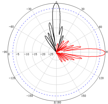
Horizontal /Vertical pattern
